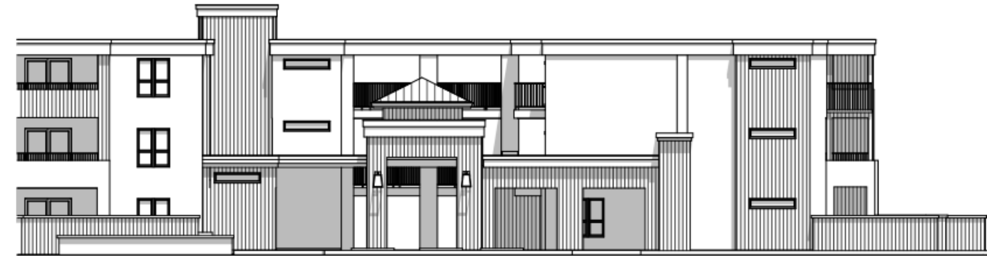
Figure 5 Draft Elevation
