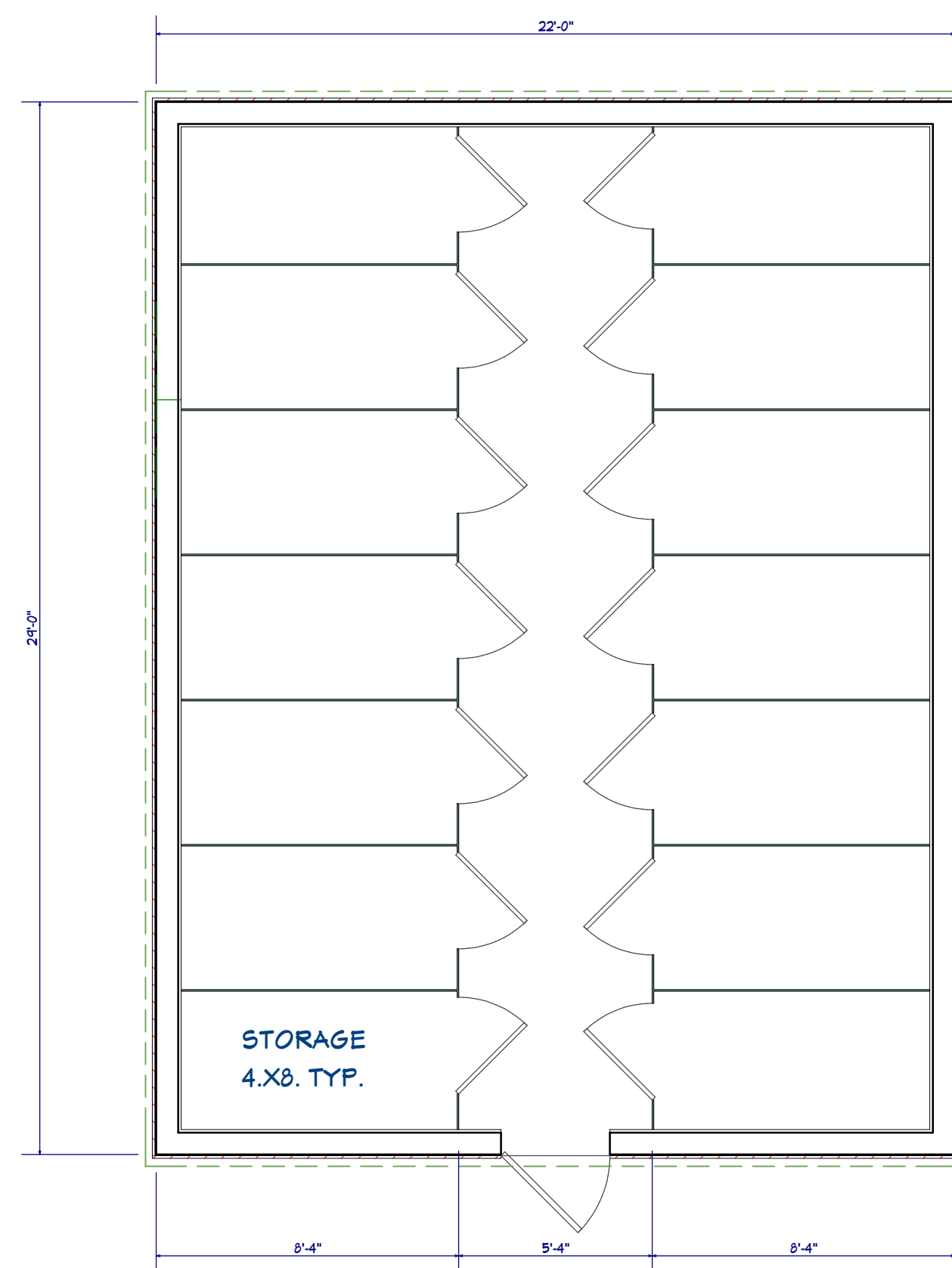
STORAGE BUILDING FLOOR PLAN
