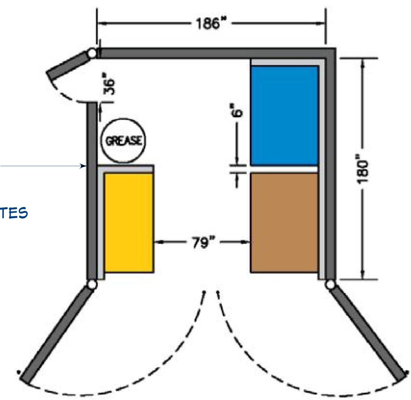
GARBAGE ENCLOSURE PLAN
