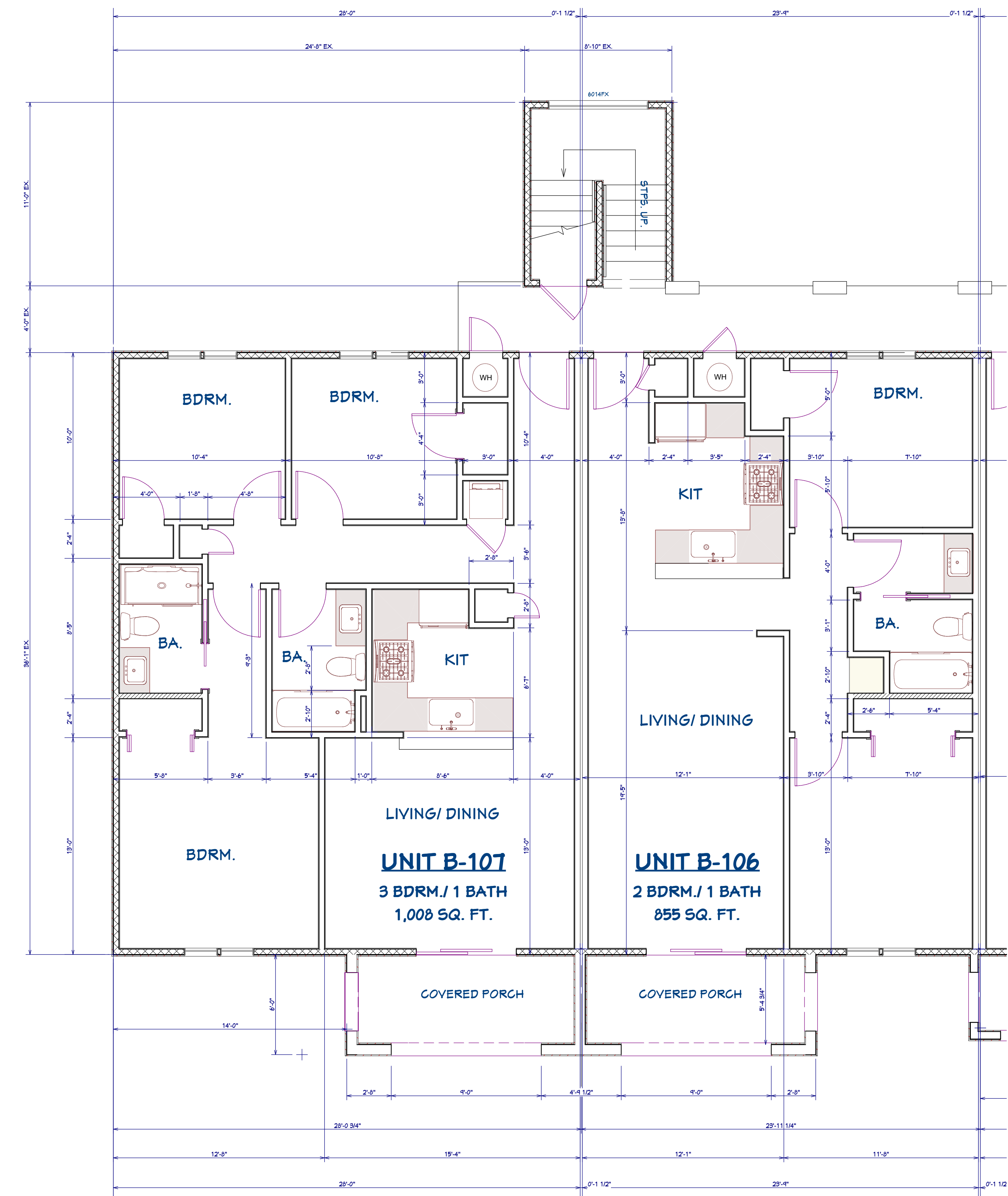
B BUILDING A & B FLOOR PLAN TYP. THREE BDRM. - TYP. TWO BDRM. 1/4"=1'-0"
