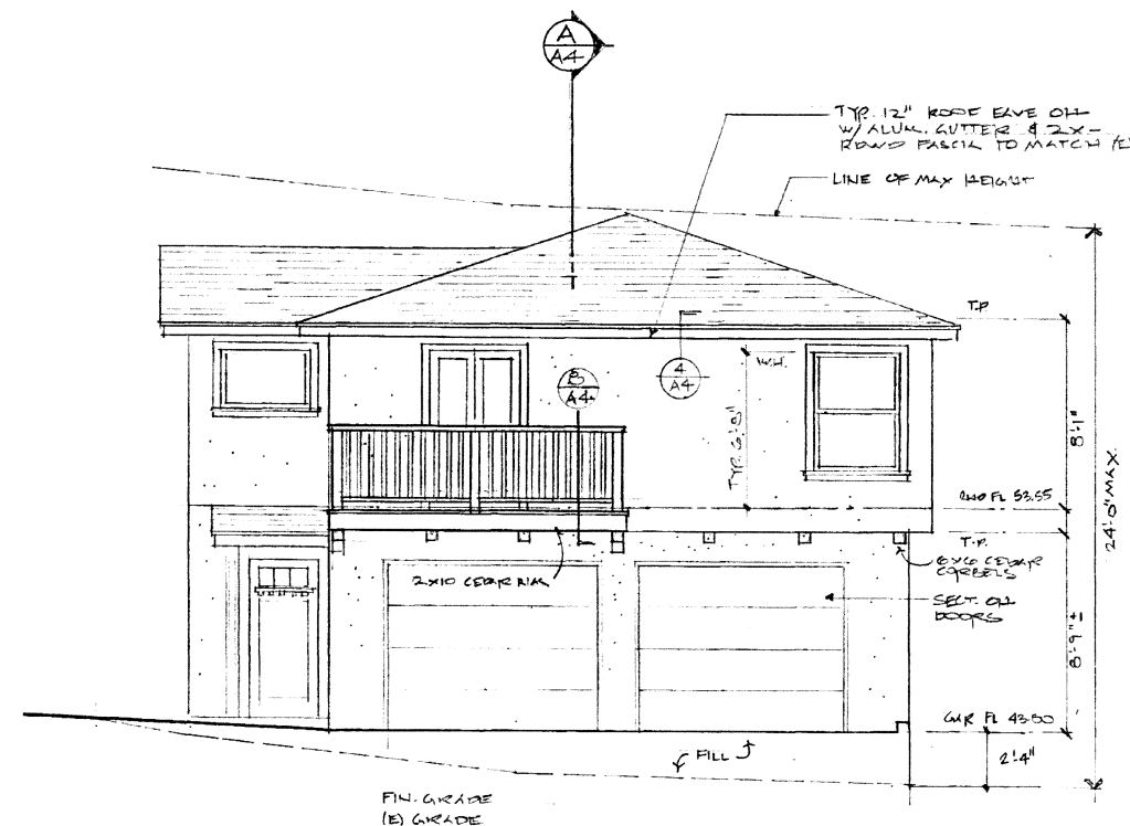
WEST ELEVATION
