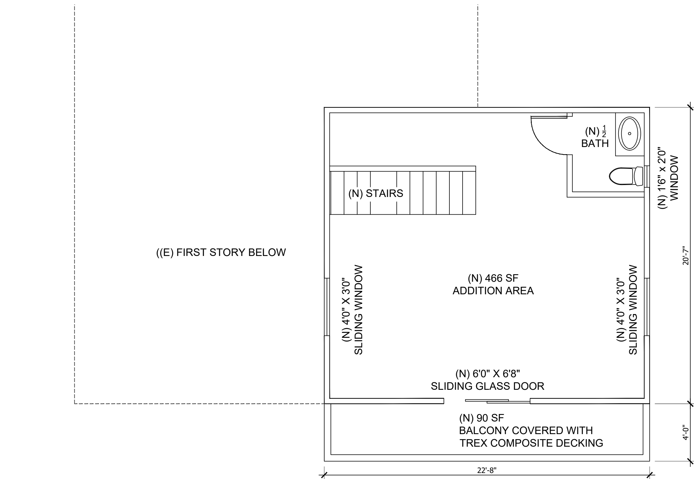
PROPOSED SECOND STORY FLOOR PLAN
