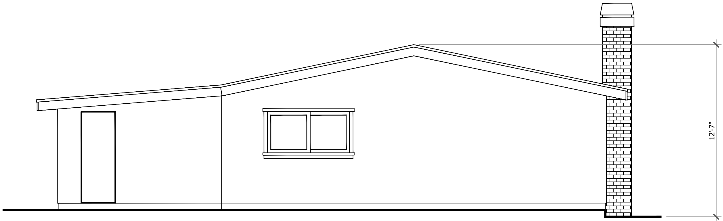
EXISTING EAST EXTERIOR ELEVATION
