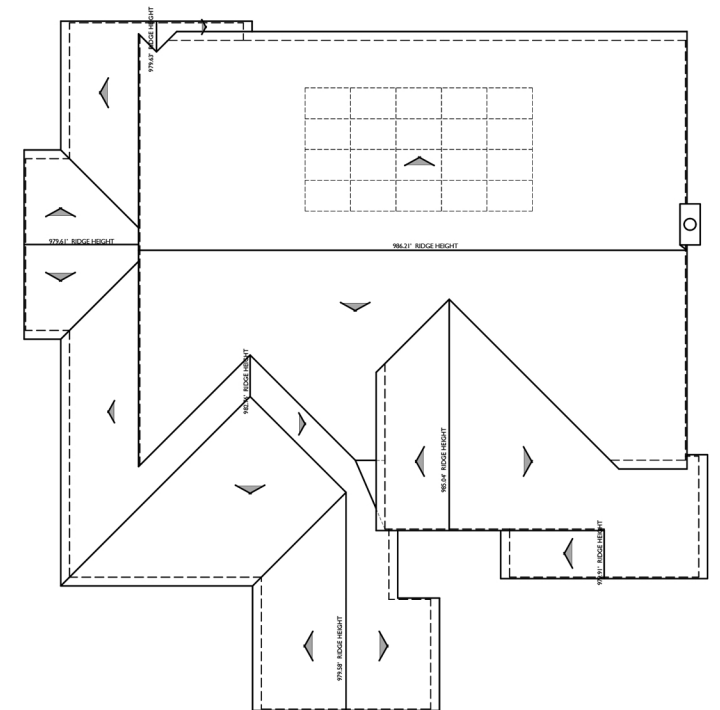
ROOF PLAN PITCH: 3.5:12 U.N.O. RAKE: 0° EAVE: 12" ROOF MATERIAL: CONCRETE 'S' TILE
