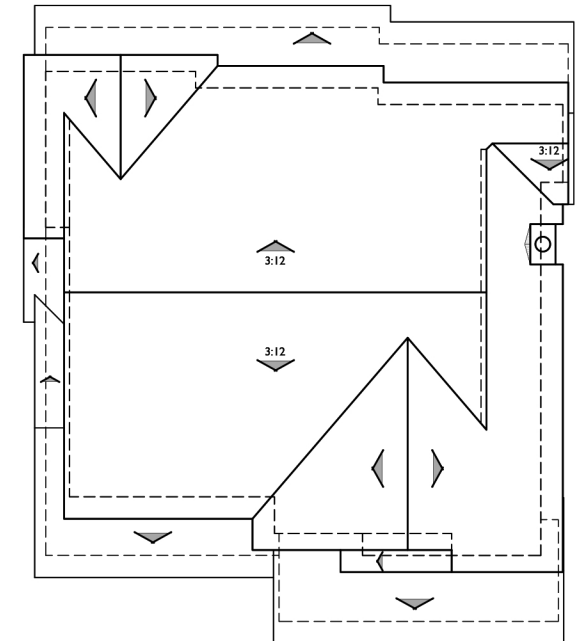
ROOF PLAN
